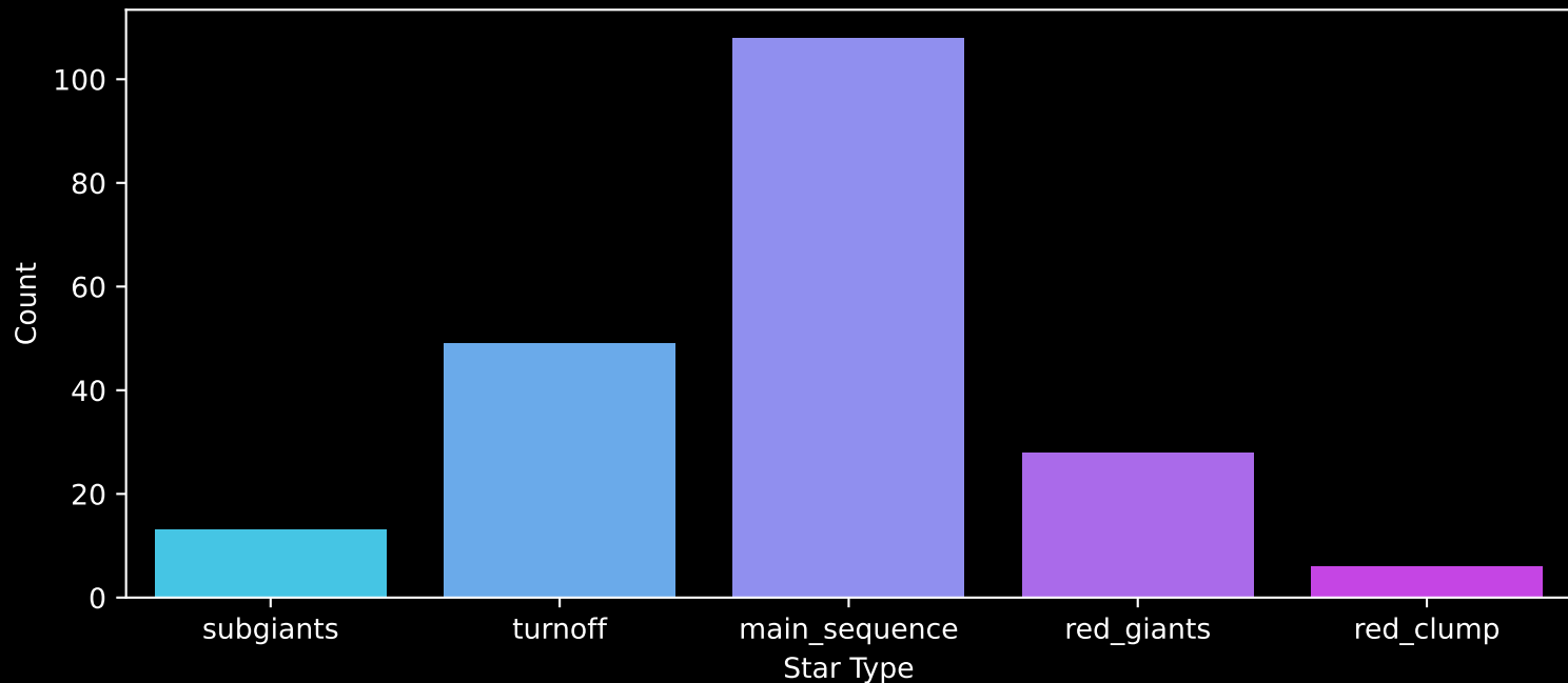
APOGEE DR17 Field: [078+52_MGA] Count plot of Star Type
