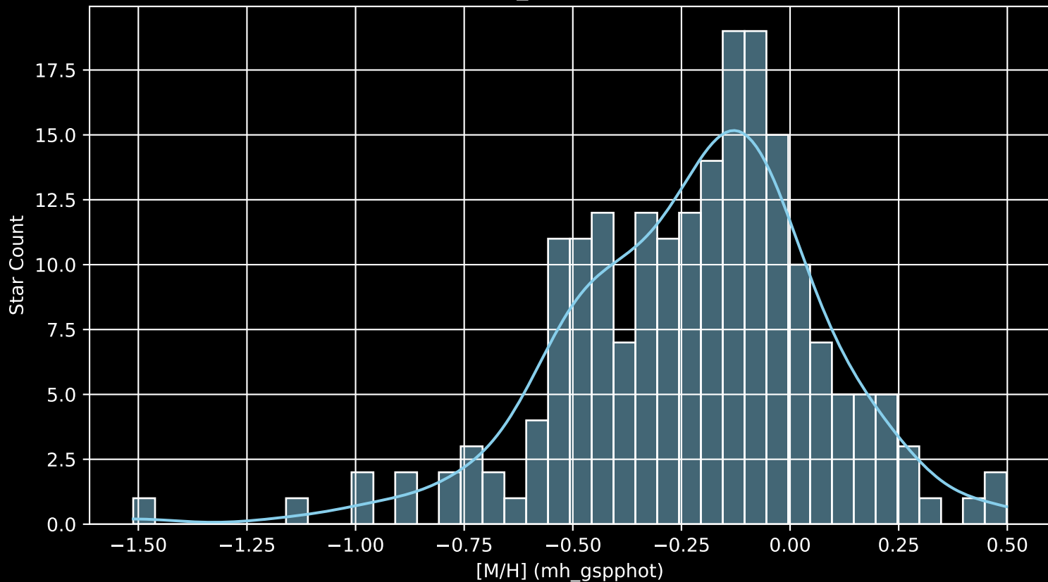
APOGEE DR17 Field: [078+52_MGA [M/H] (mh_gspphot) (n= 200)
