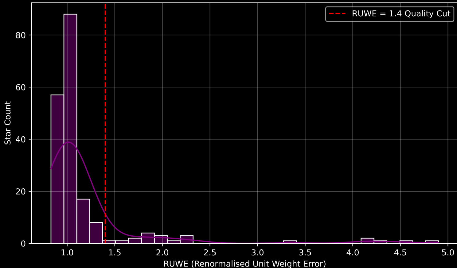
GAPOGEE DR17 Field [078+52_MGA] RUWE Distribution (n= 191)
