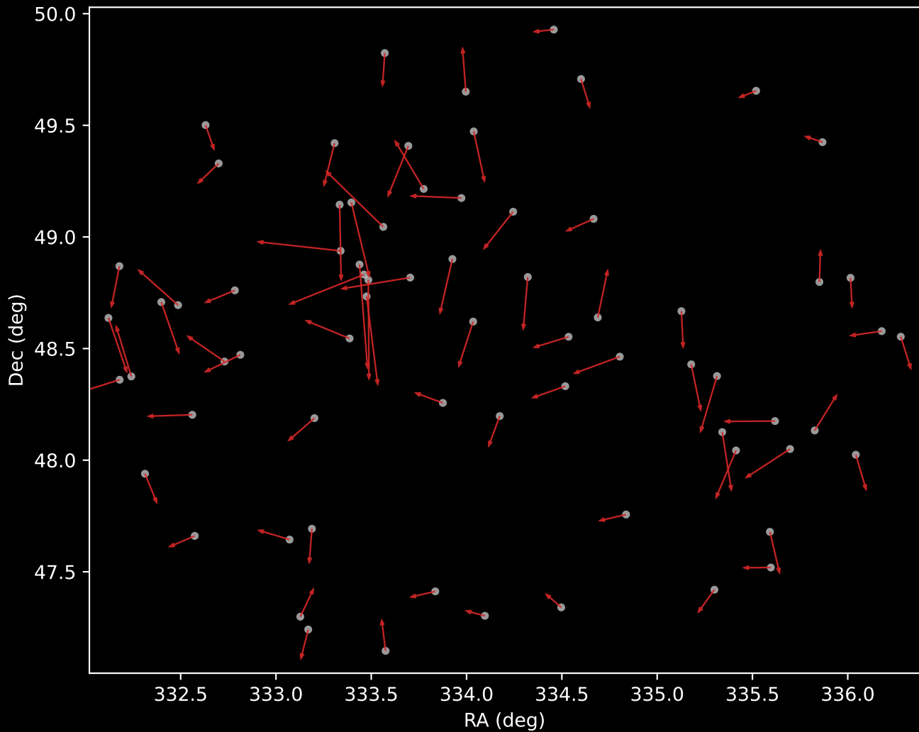
APOGEE DR17 Cluster 6 Proper Motion Vectors (n=72)
