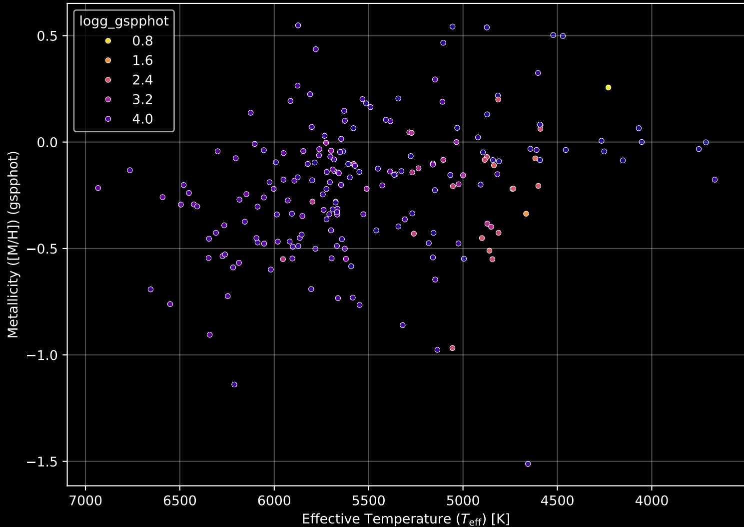
APOGEE DR17 Field: [078+52_MGA] Stellar Population Parameters (n= 204)
