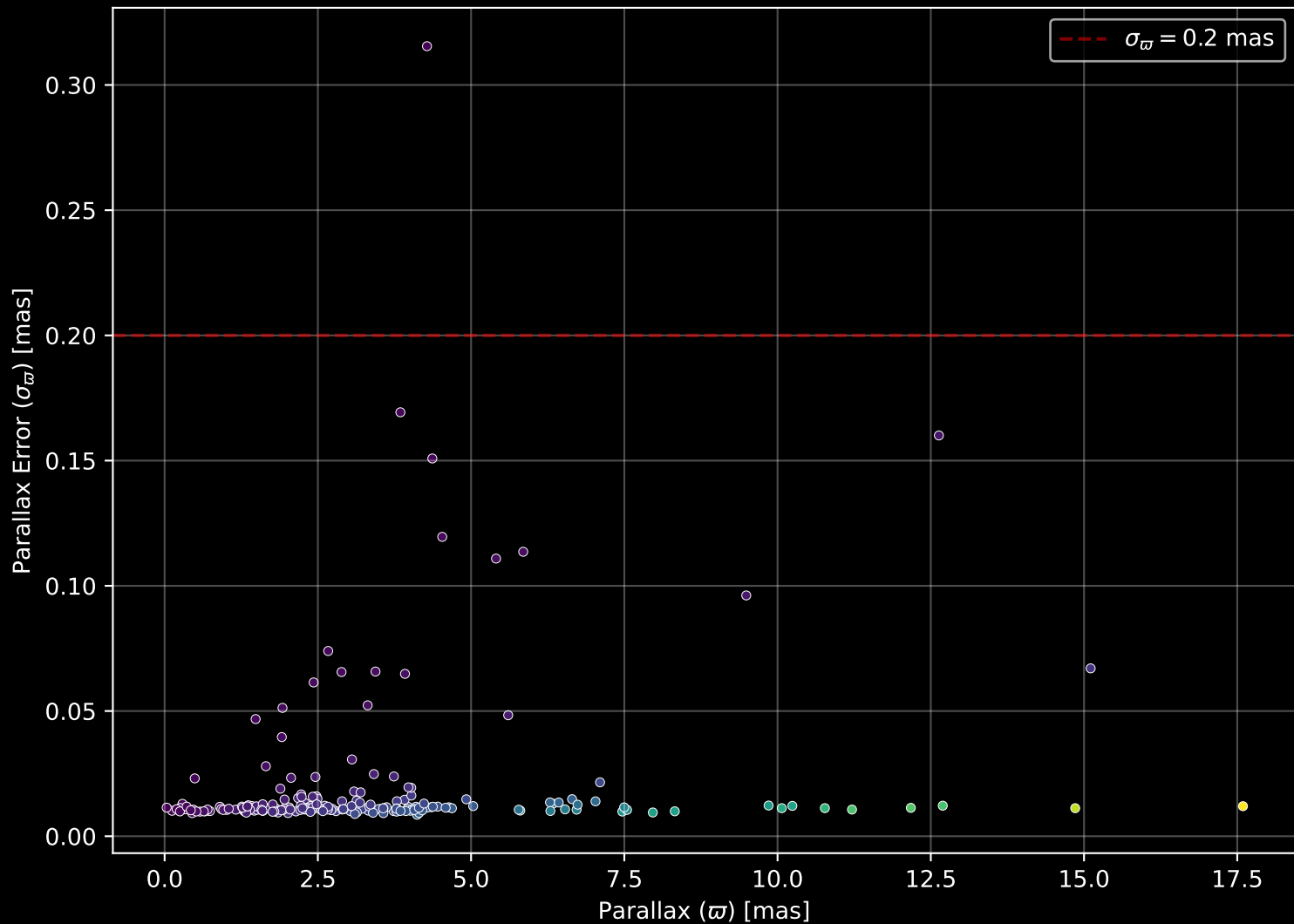
APOGEE DR17 Field: [078+52_MGA] Parallax Quality (n= 204)
