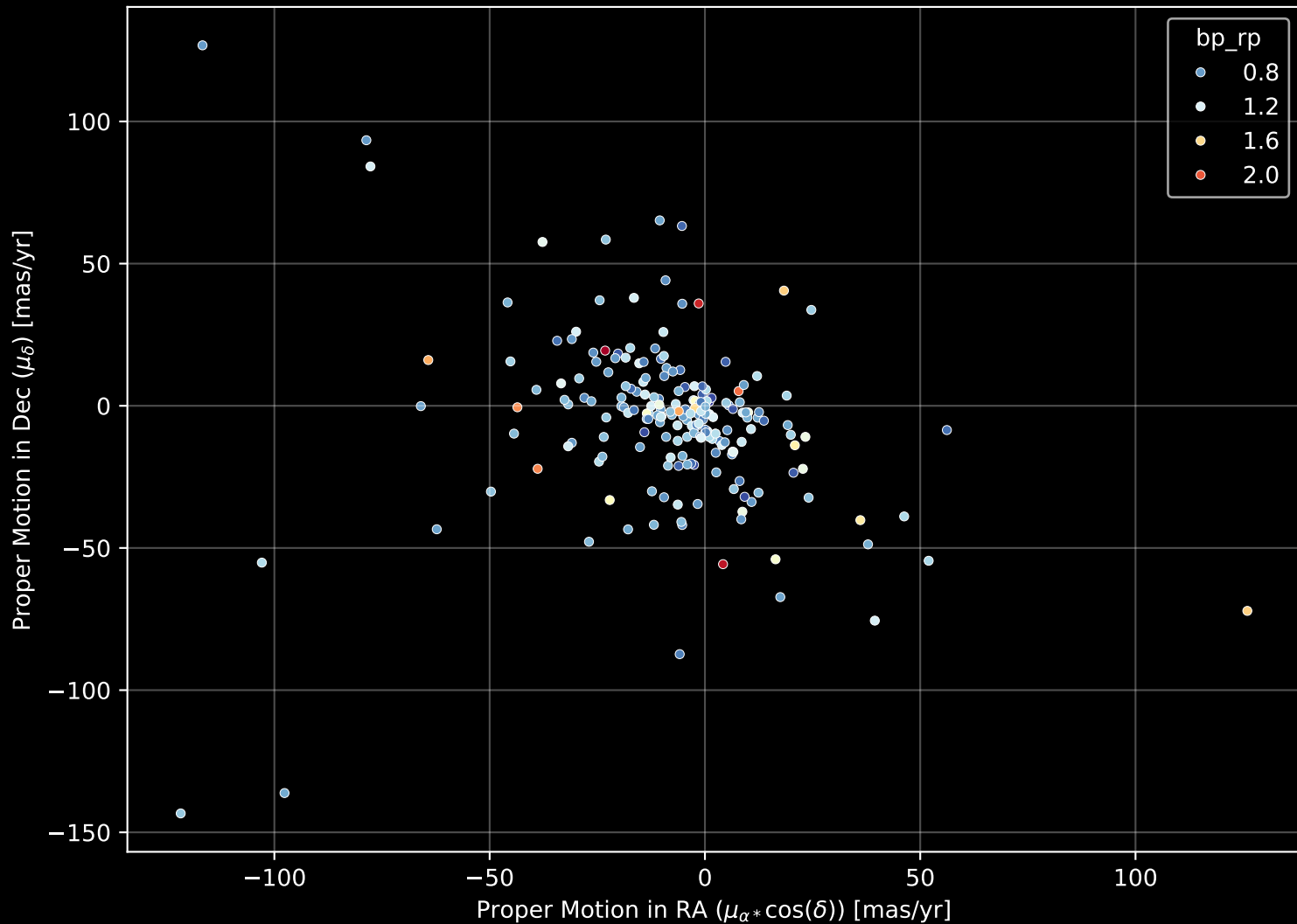
APOGEE DR17 Field: [078+52_MGA] Proper Motion Diagram (n= 204)
